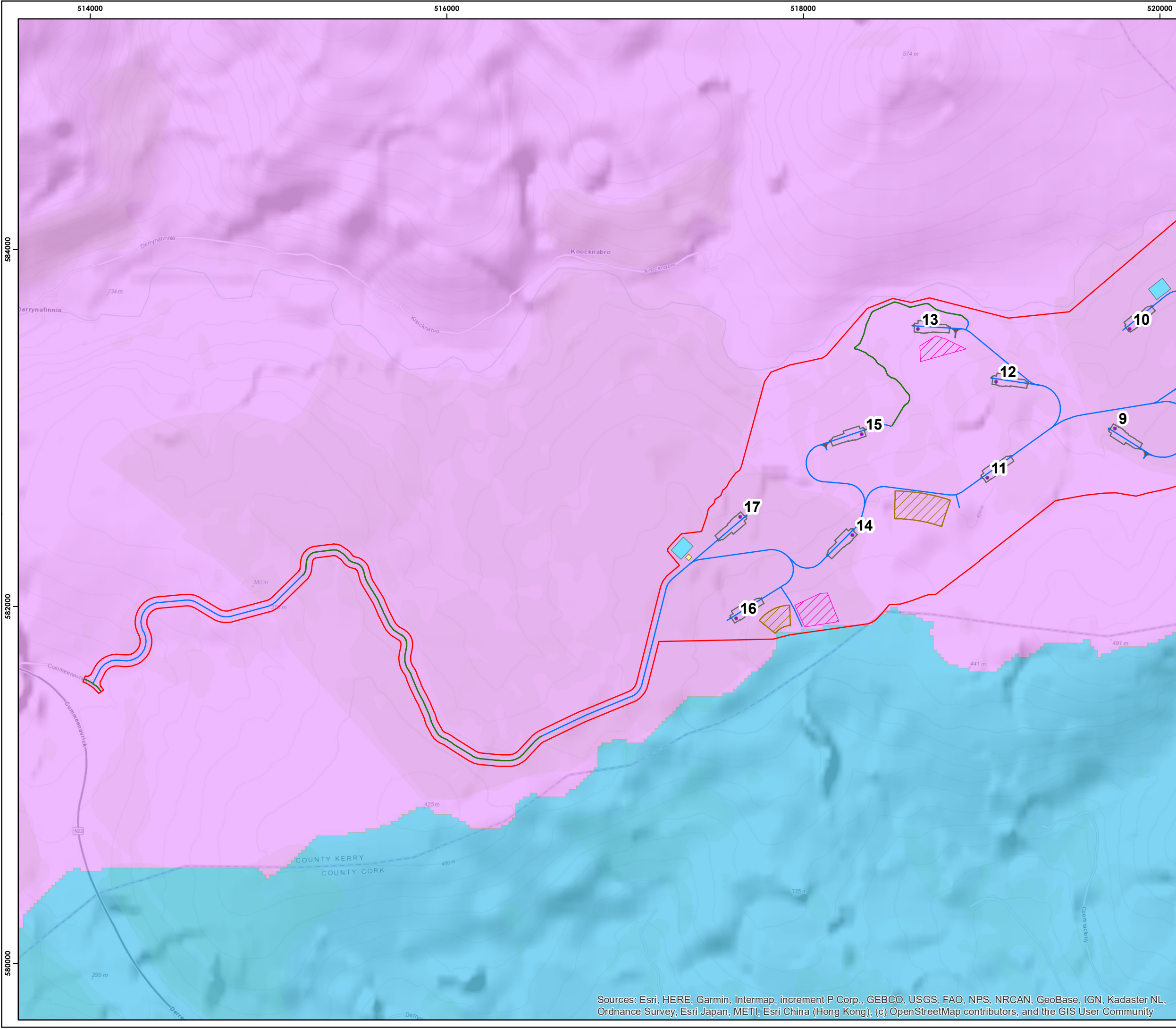
Figure10-4a Groundwater Bodies
